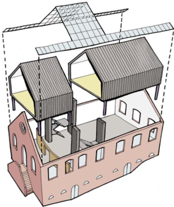
Exploded view
